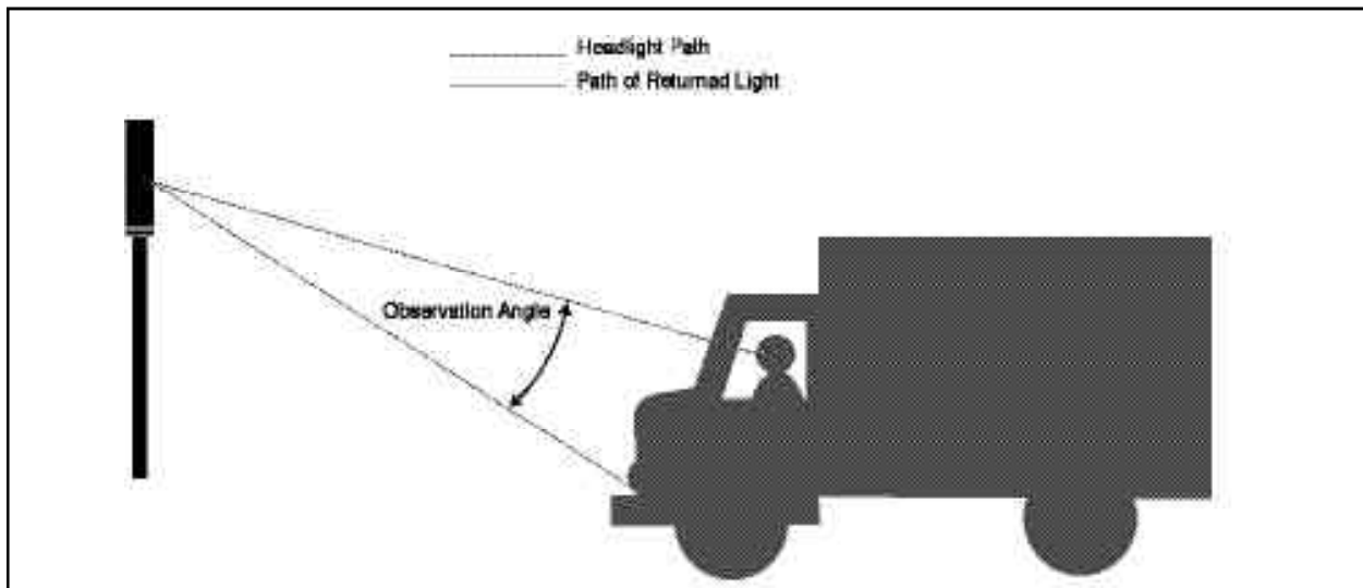
Figure 3.3 – Observation Angle
