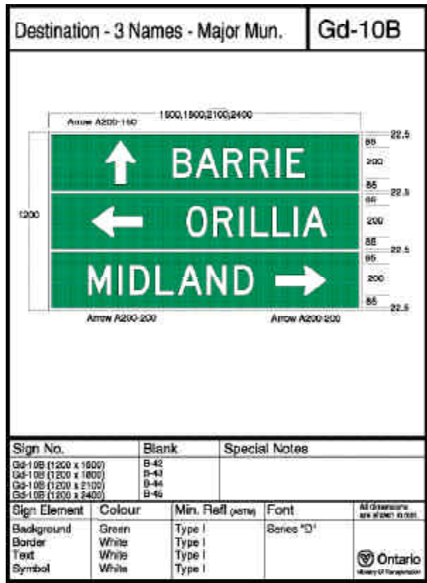
Figure 5.2 – Sign Pattern Template for Gd-10B
