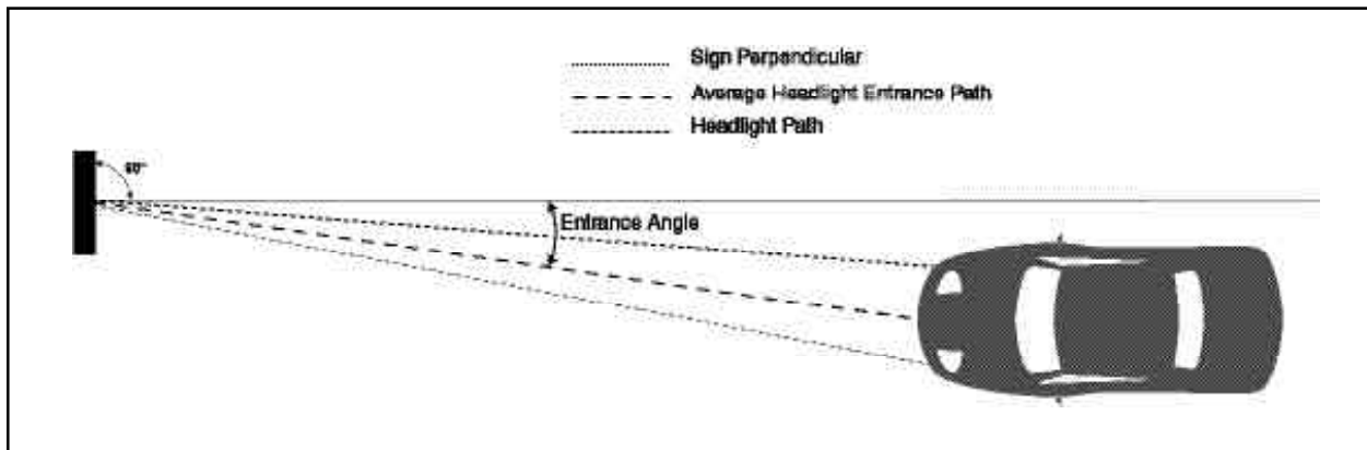
Figure 3.2 – Entrance Angle
